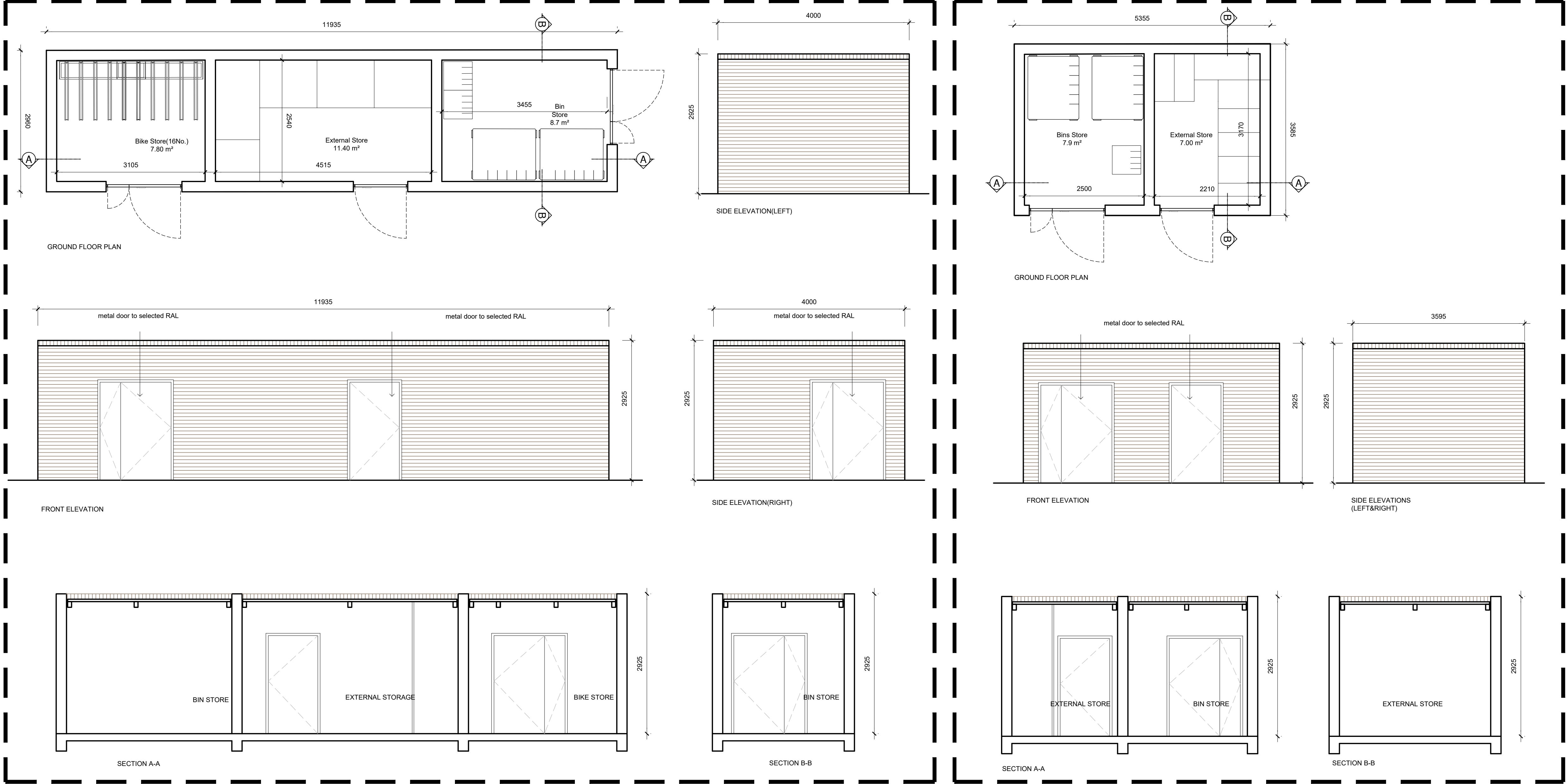
BIN STORE, BICYCLE STORE & EXTERNAL STORAGE TYPE 1
